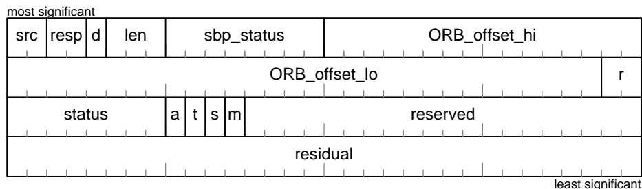
Figure 9 – Status block format
