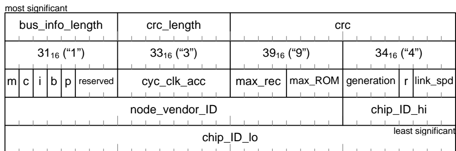
Figure 14 – First five quadlets of configuration ROM
